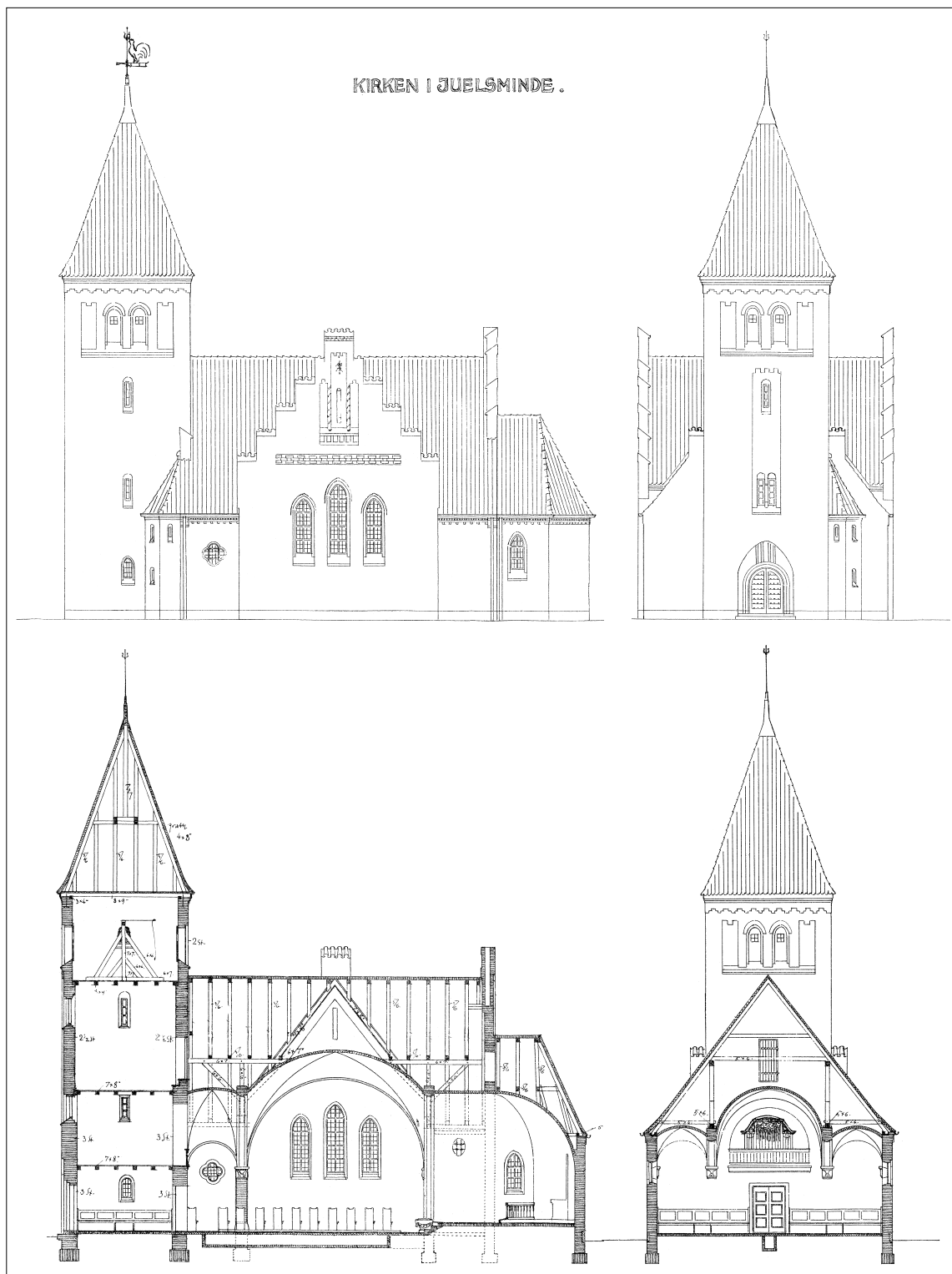
Fig. 2. Opstalter og snit. 1:300. Forslag til kirken, tegnet af Johs. Magdahl Nielsen 1911. – Elevations and Sections. Proposal for the church drawn by Johs. Magdahl Nielsen in 1911.
