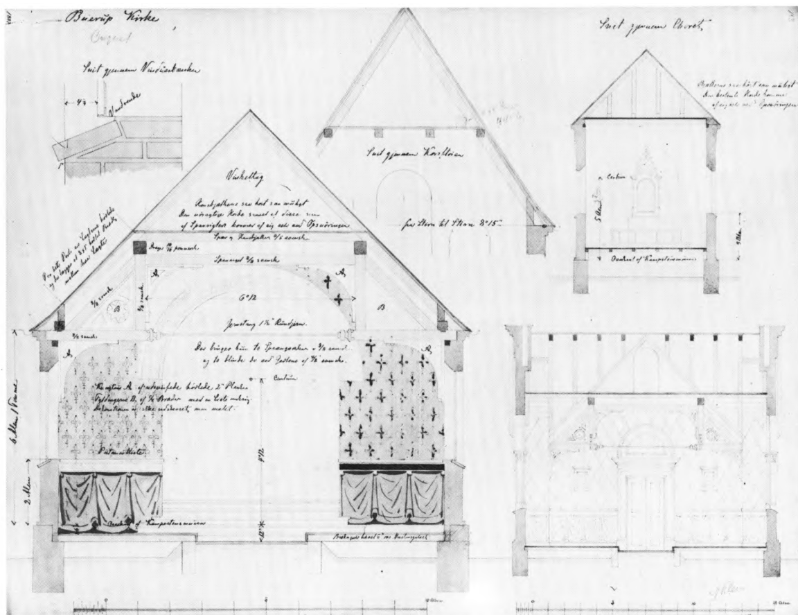
Fig. 1. Tværnsnit i kor, skib og korsarm. Farvelagt blad, signeret V. Klein 1887. Kunstakademiets Bibliotek. - Cross-sections of chancel, nave and crossing. Coloured leaf signed »V Klein 1887«.
